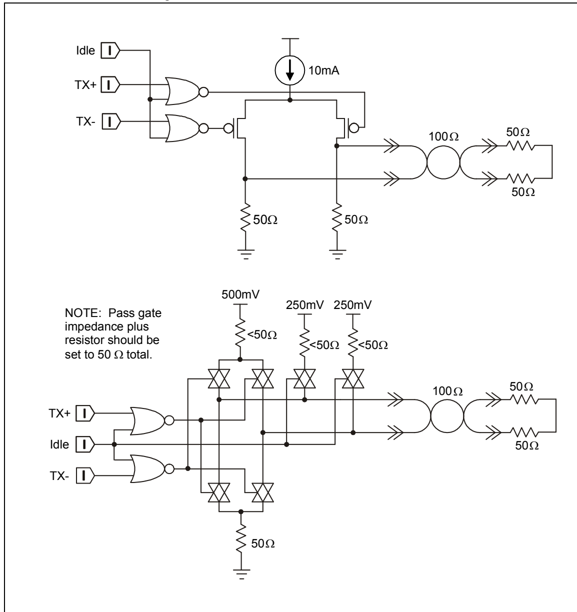
Figure 181 – Transmitter Examples
