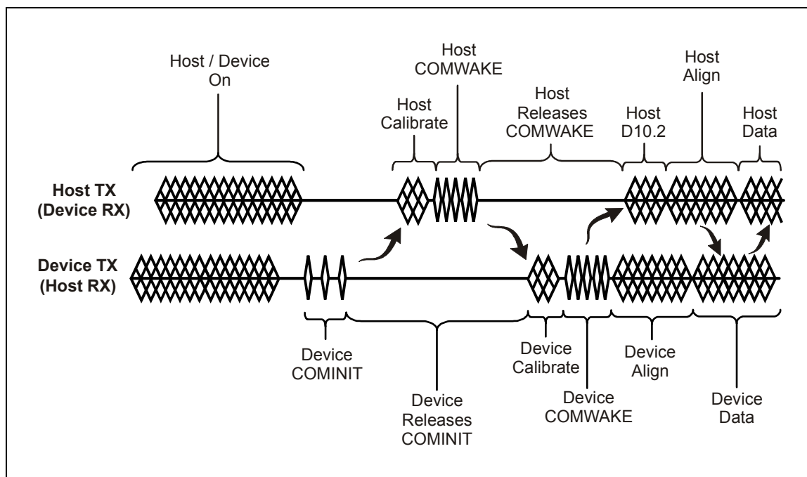
Figure 184 – COMINIT Sequence
