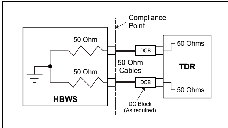
Figure 173 – TDR Differential Impedance Test—Setting Risettime
