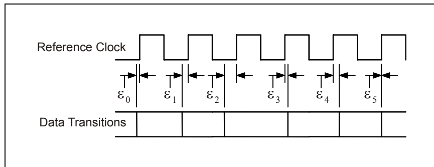
Figure 271 – Jitter Deviations
