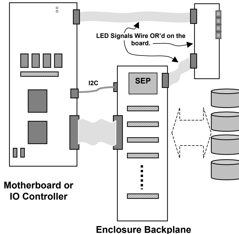
Figure 245 – Device Activity LEDs in a Storage Subsystem
