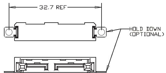
Figure 75 - Slimline Device Plug Connector Optional Hold Down Mounting
