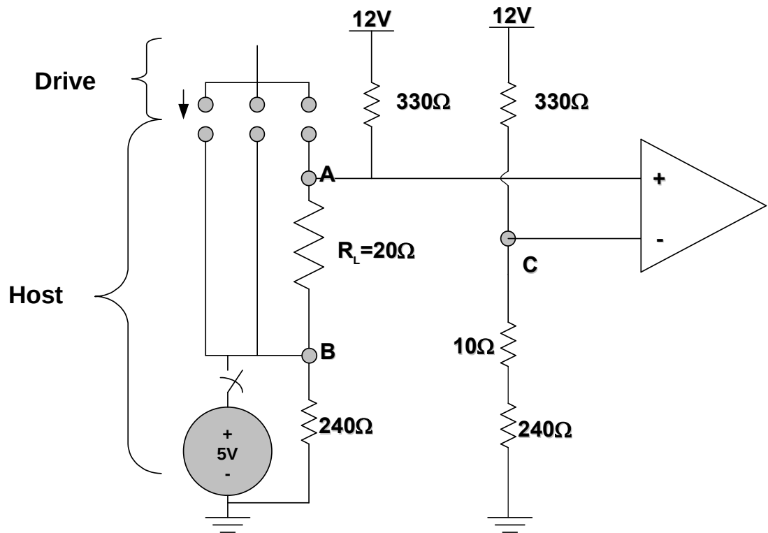
Figure 110 – Example presence detection implementation
