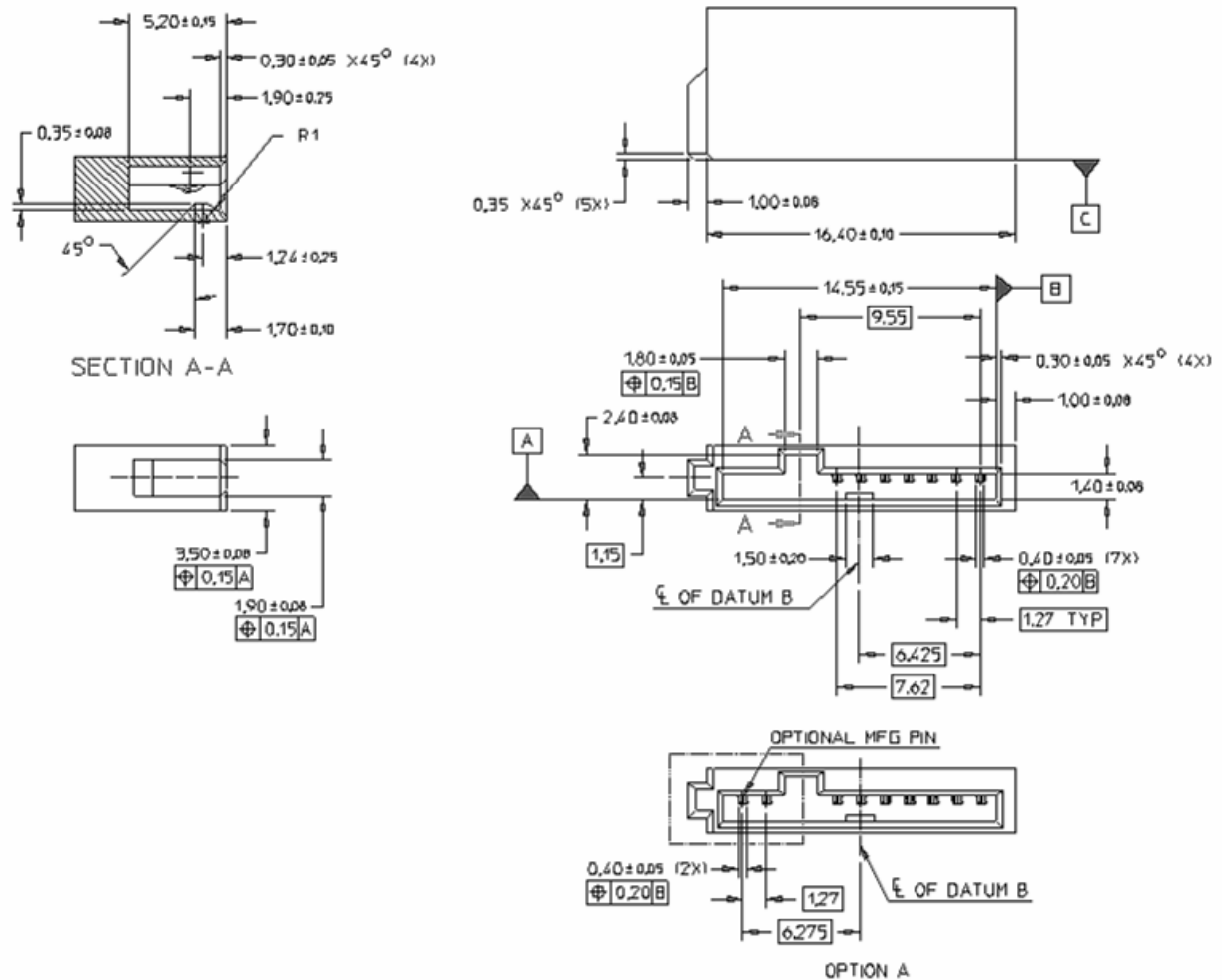
Figure 57 Internal micro SATA power receptacle connector
