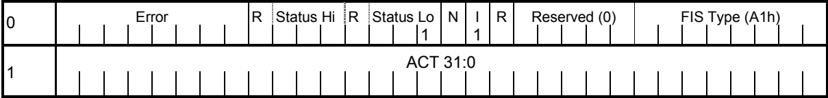
Figure 216 - NCQ QUEUE MANAGEMENT, Abort NCQ Queue – error during execution
