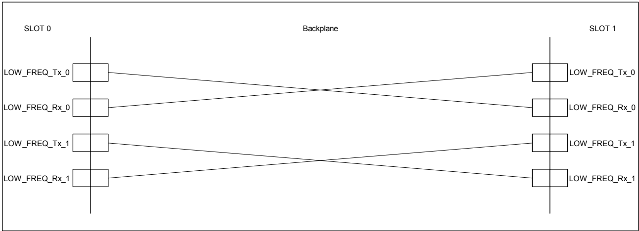
Figure 263 – Low Speed Channels
